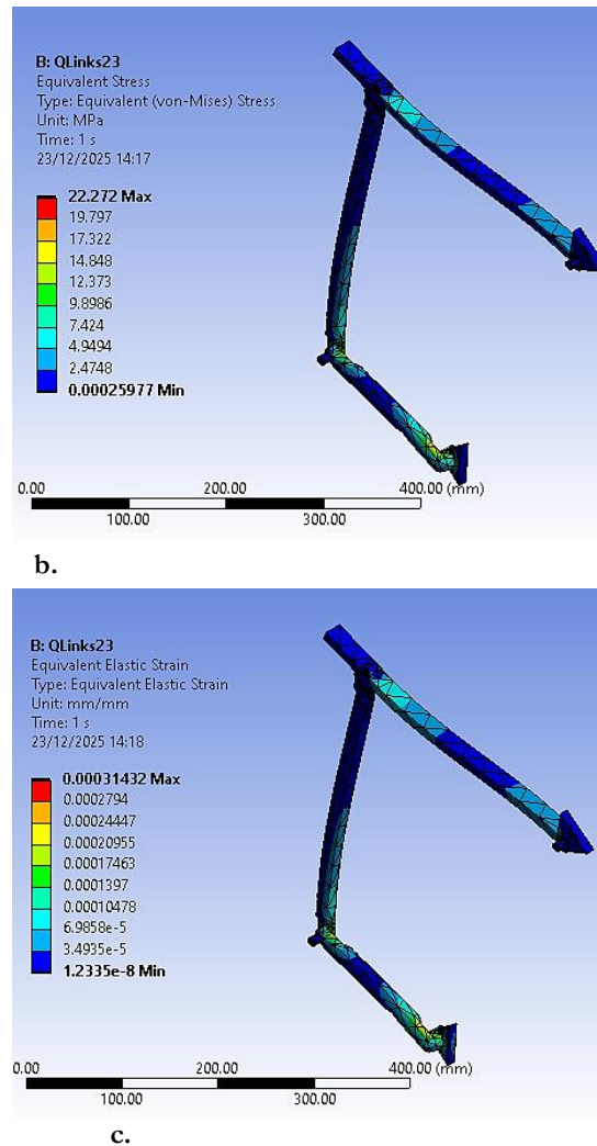
Fig. 8. Structural integrity of the swing board mechanism; a. structural displacement, b. stress analysis, and c. equivalent strain.
