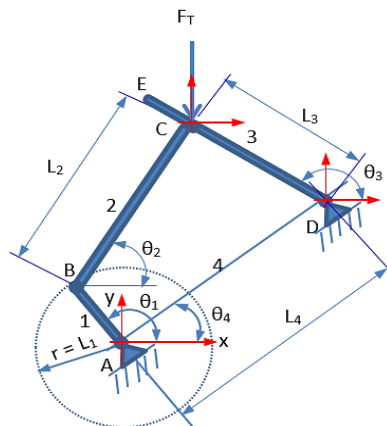
Fig. 2. Four-bar link mechanism for patient recuperating exercise.
