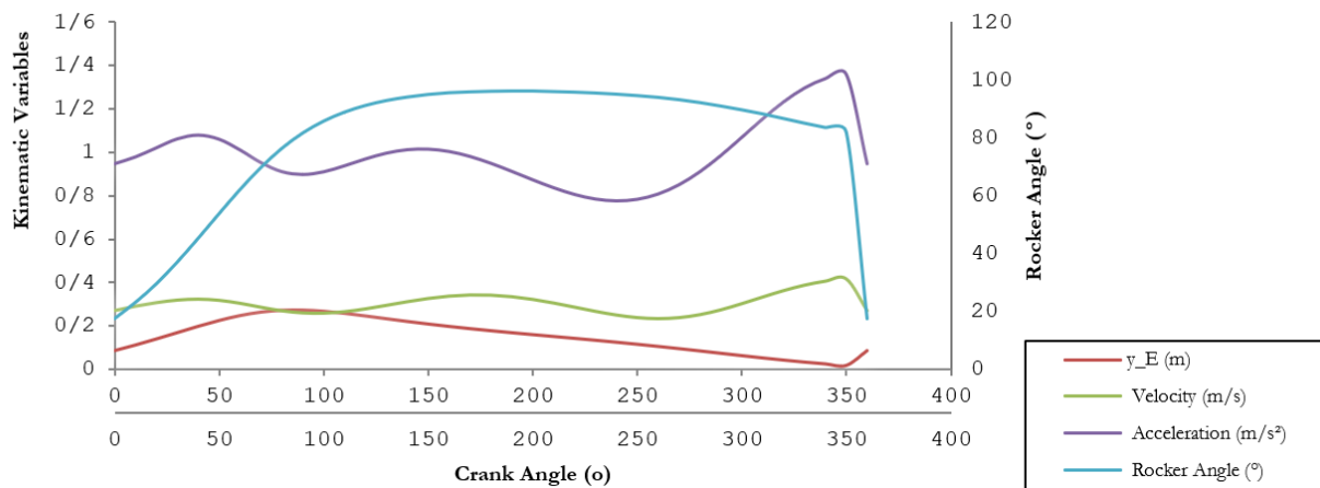
Fig. 4. Initial kinematic profile over a complete cycle of the swing-board.
