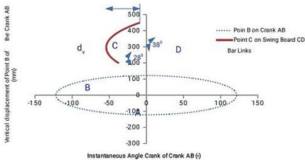
Fig. 5. Loci of points B of the crank and point c of the swing-board.
