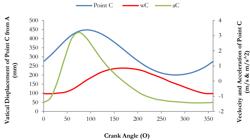
Fig. 6. Position, velocity and acceleration of point c in the link mechanism.
