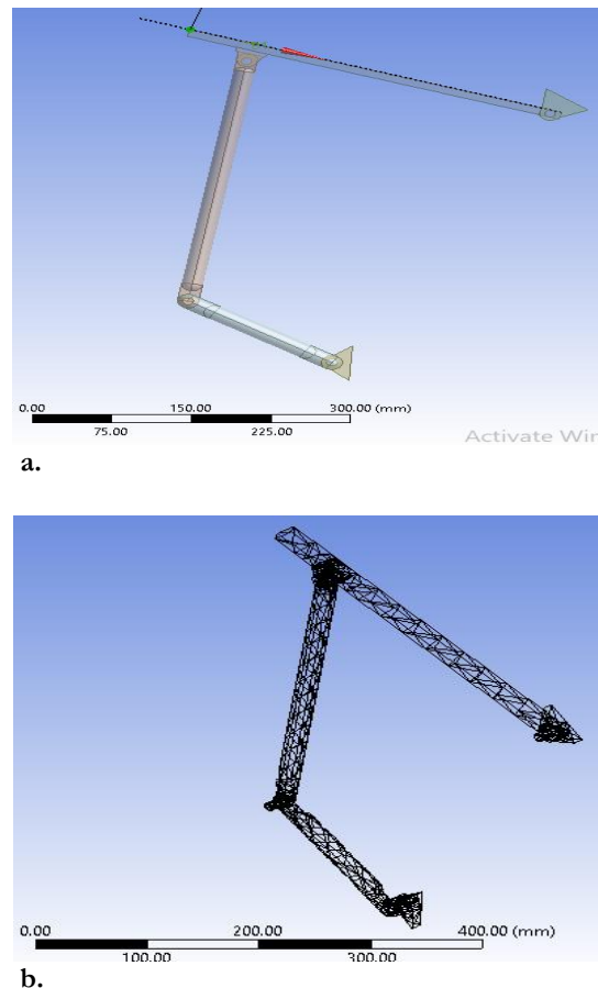
Fig. 3. Preparing the link mechanism for Static force and stress analysis.
