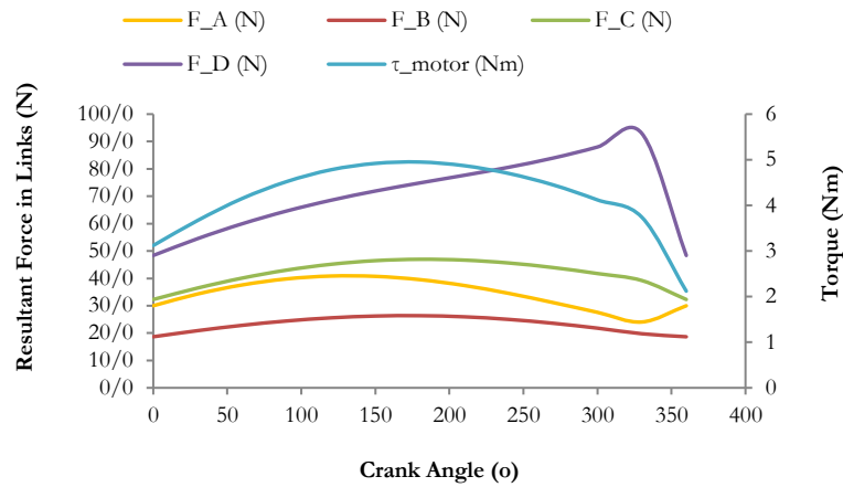
Fig. 7. Resultant forces in bar links and torque in the crank.
