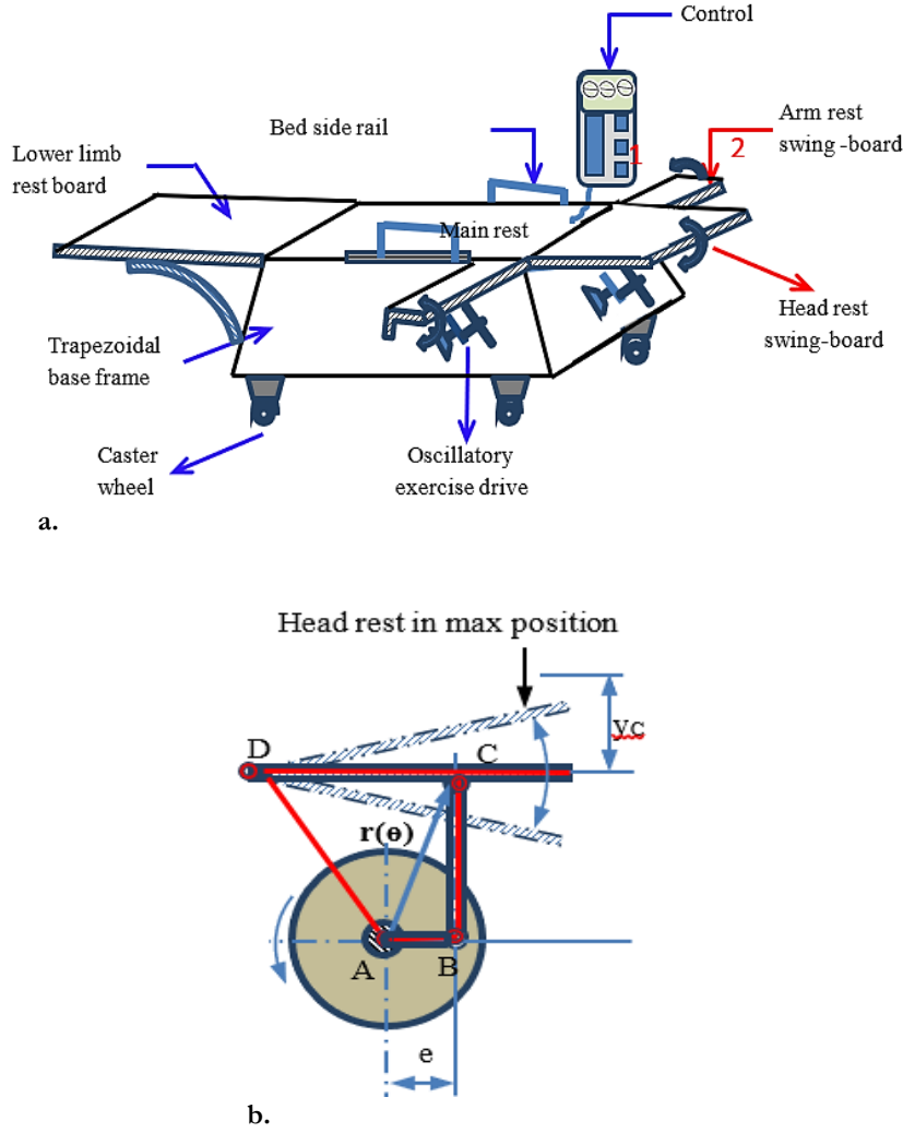
Fig. 1. Schematic of the model concept for an automated patient bed for exercise; a. bed assembly, and b. 4-bar link mechanism the exercise board swings.
