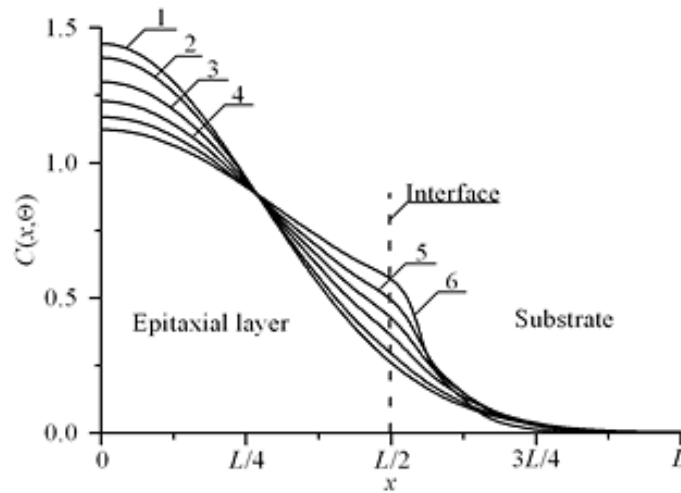
Fig. 2. Dopant concentration profiles in the heterostructure.
