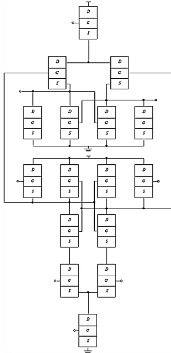
Fig. 1. The considered comparator [15].
