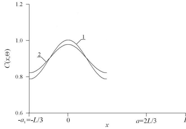
Fig. 4. Distributions of concentration of dopant.
