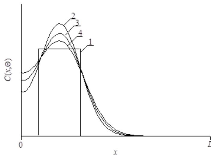
Fig. 7. Distributions of concentration of implanted dopant in depth of heterostructure.
