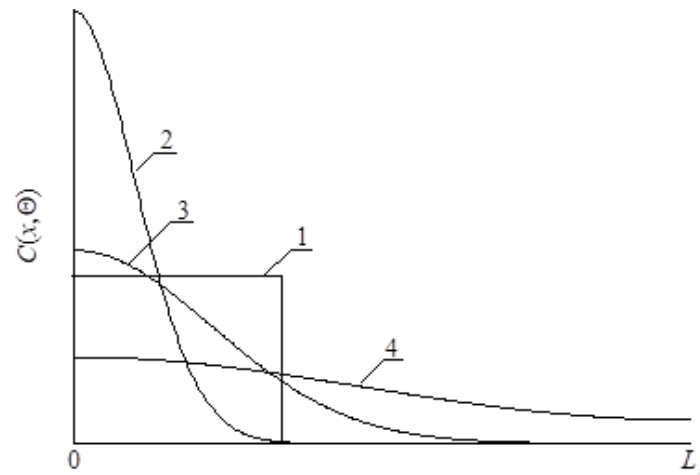
Fig. 6. Distributions of concentration of infused dopant in depth of heterostructure.
