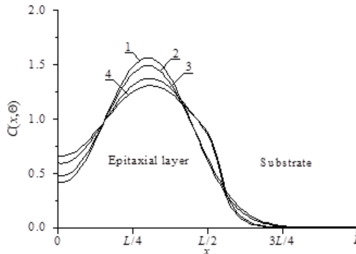
Fig. 3. Dependences of concentration of dopant, implanted in heterostructure.
